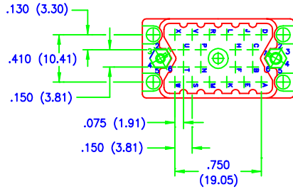
20 PIN PLUG
