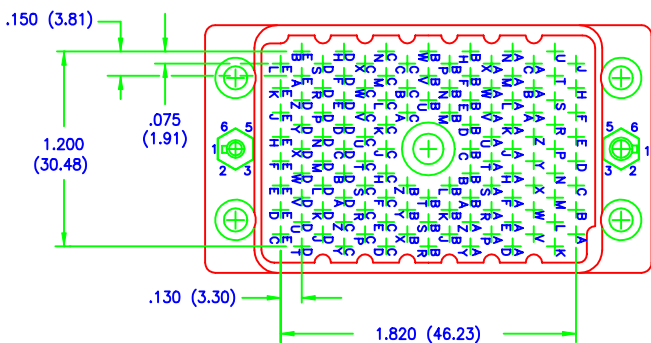
120 PIN PLUG
