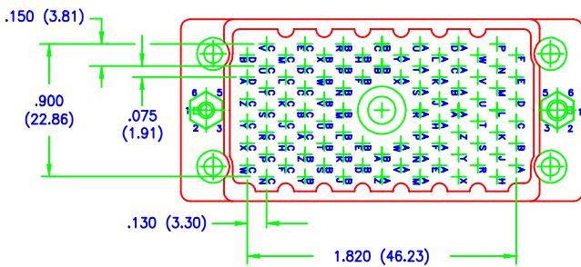
90 PIN PLUG
