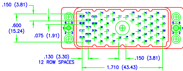
56 PIN PLUG
