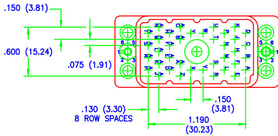
38 PIN PLUG
